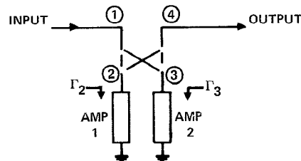
Figure 2a. Hybrid coupled amplifier with different reflection networks or different diodes.
