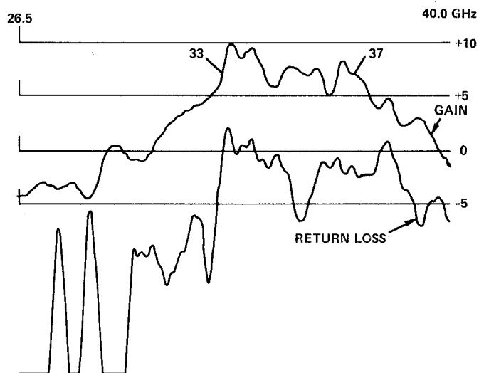
Figure 6. Four diode amplifier tuned for maximum gain-bandwidth.
